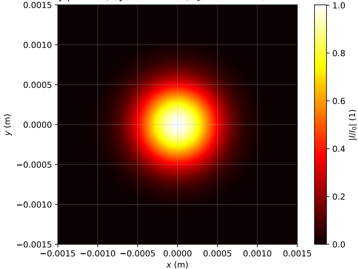
Intensity profile I(x, y, z = 0.080\text{m})/I_0 , \text{Pin}=0.5\text{Pcr} , artificial time
